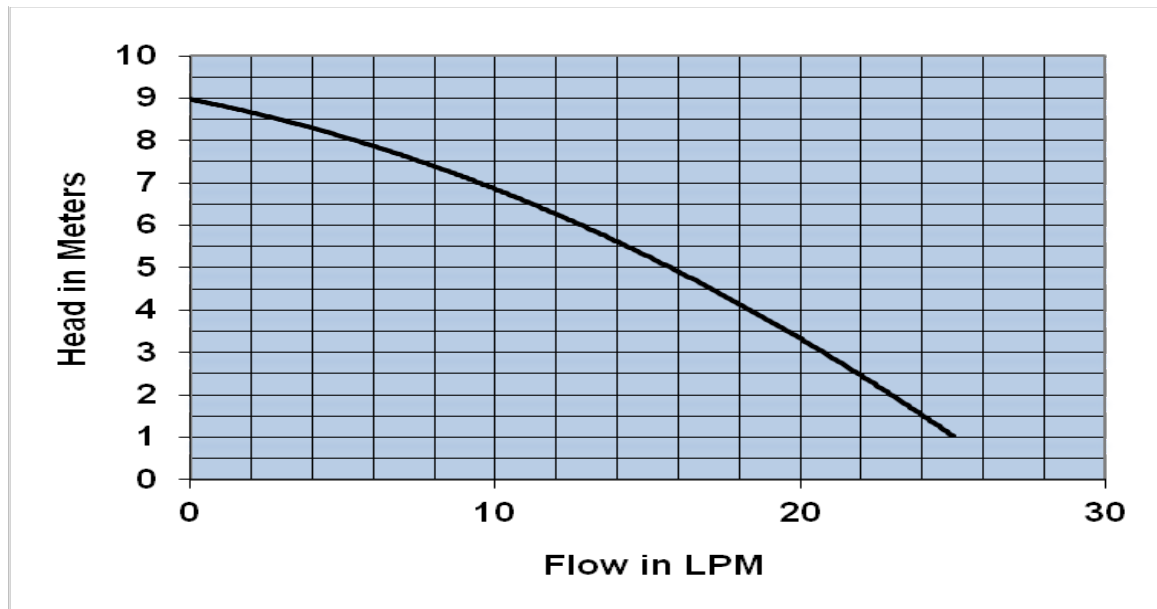
Flow Performances
