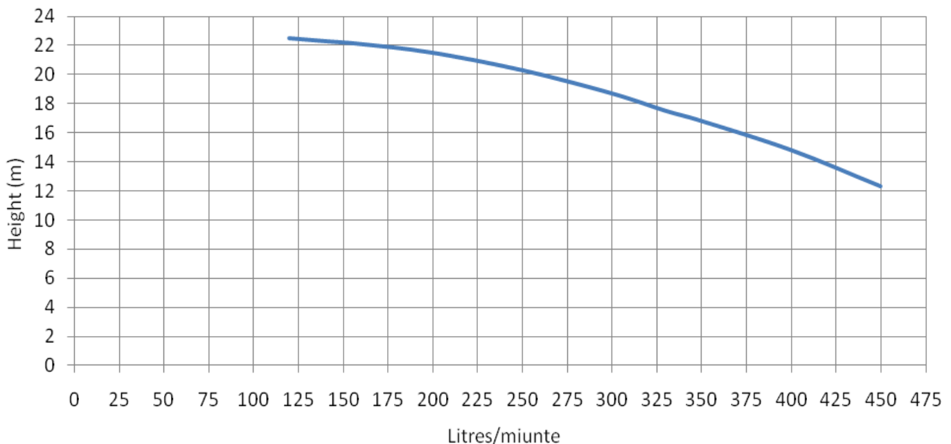
Pump Performance
