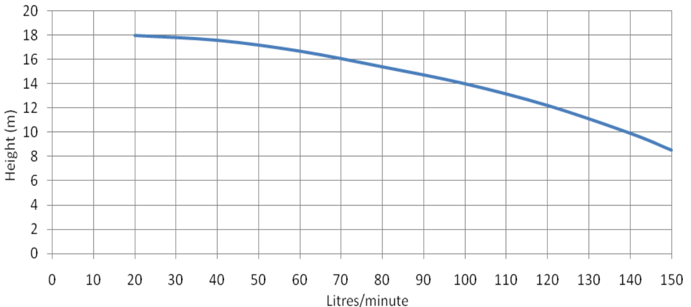
Pump Performance
