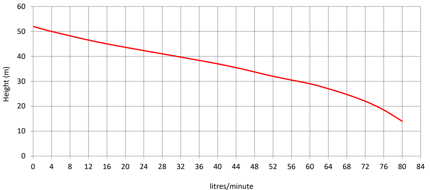
Pump Performance
