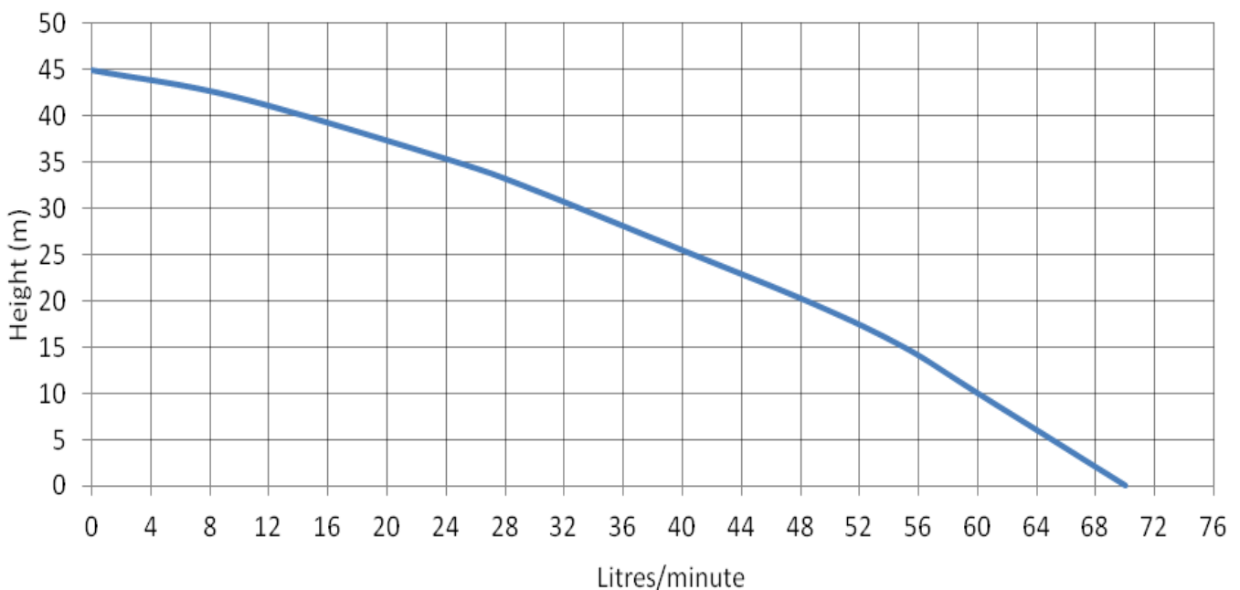
Pump Performance
