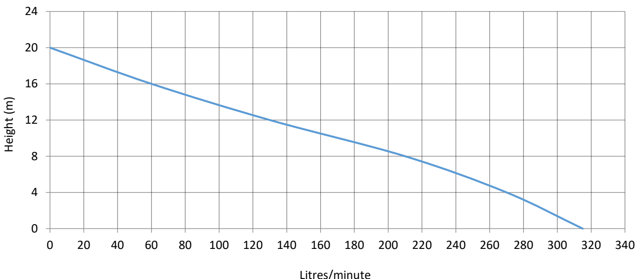
Pump Performance
