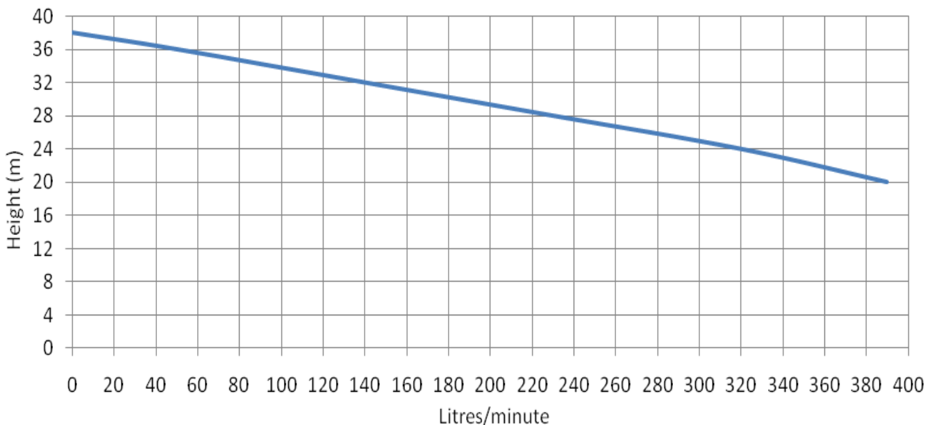
Pump Performance
