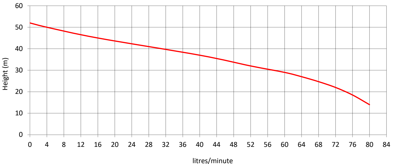
Pump Performance
