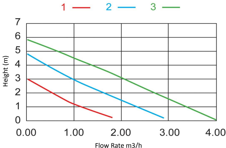
Pump Performance (3 x Speeds)
