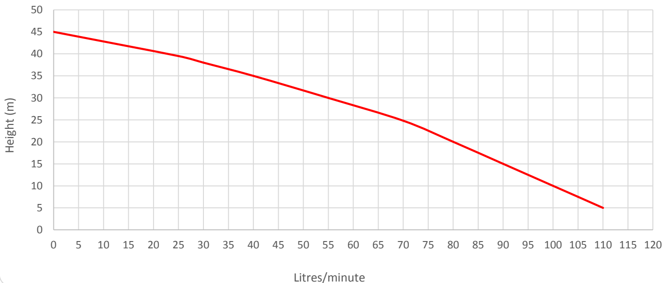
Pump Performance
