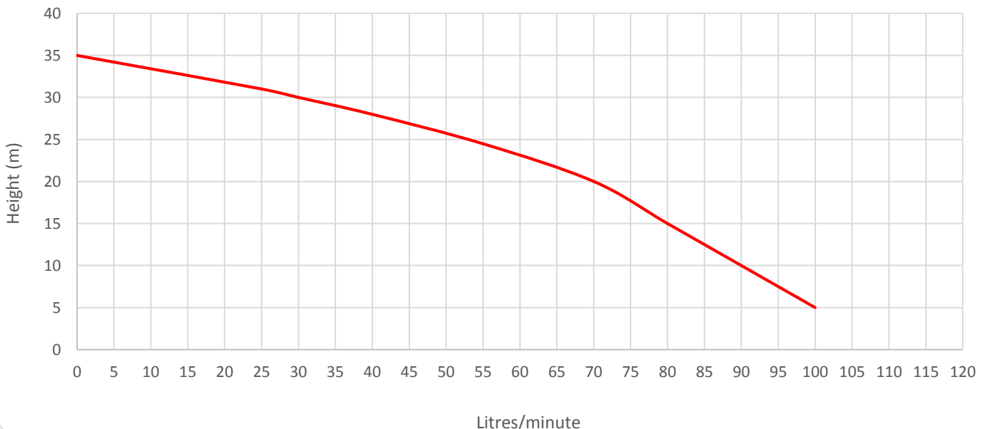
Pump Performance
