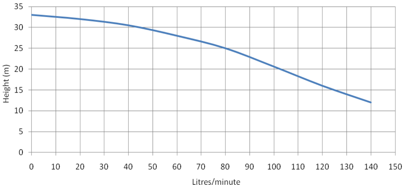
Pump Performance
