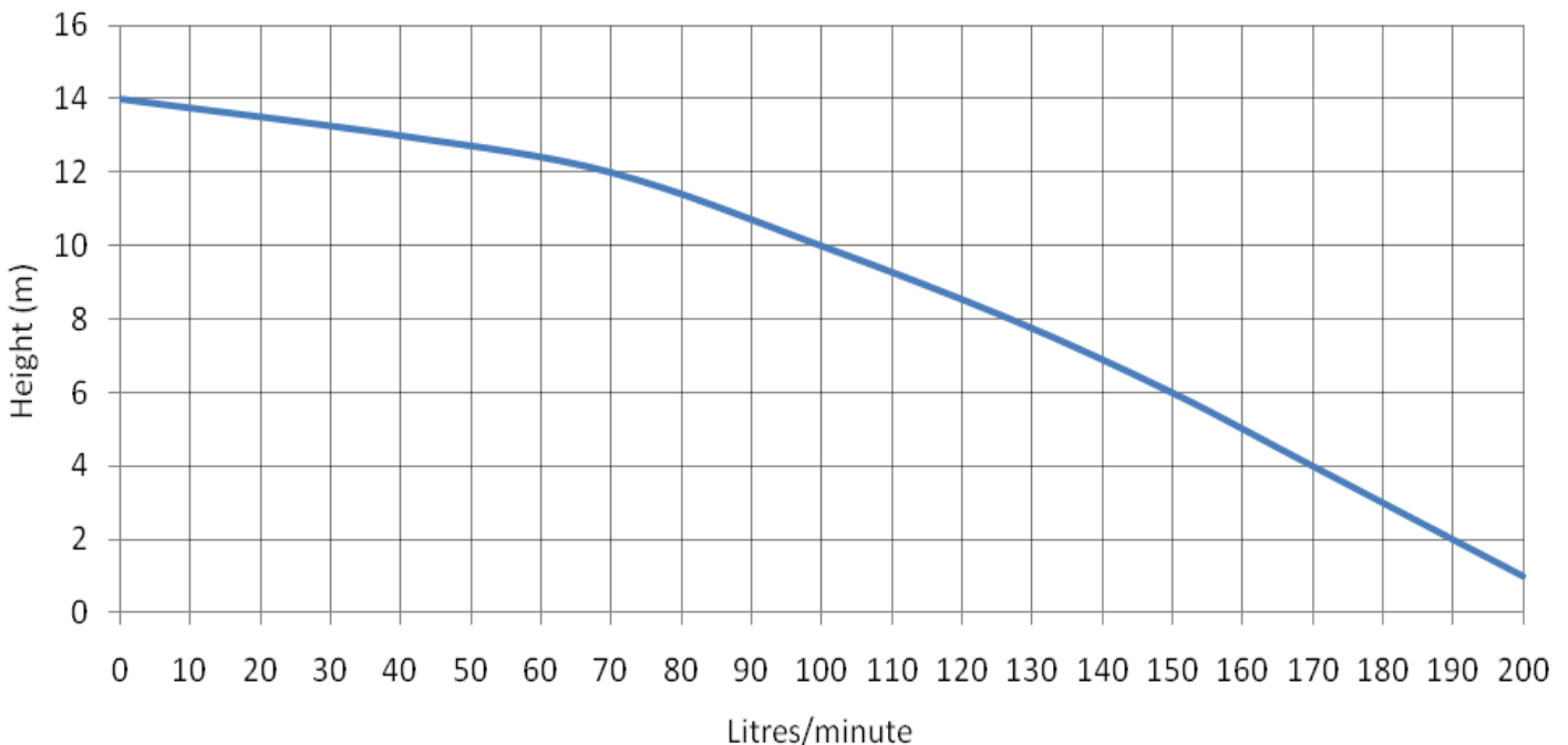
Pump Performance
