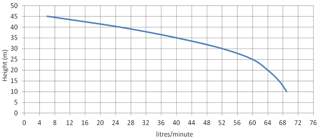
Pump Performance
