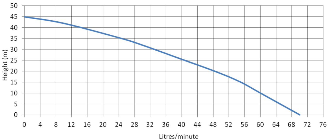
Pump Performance
