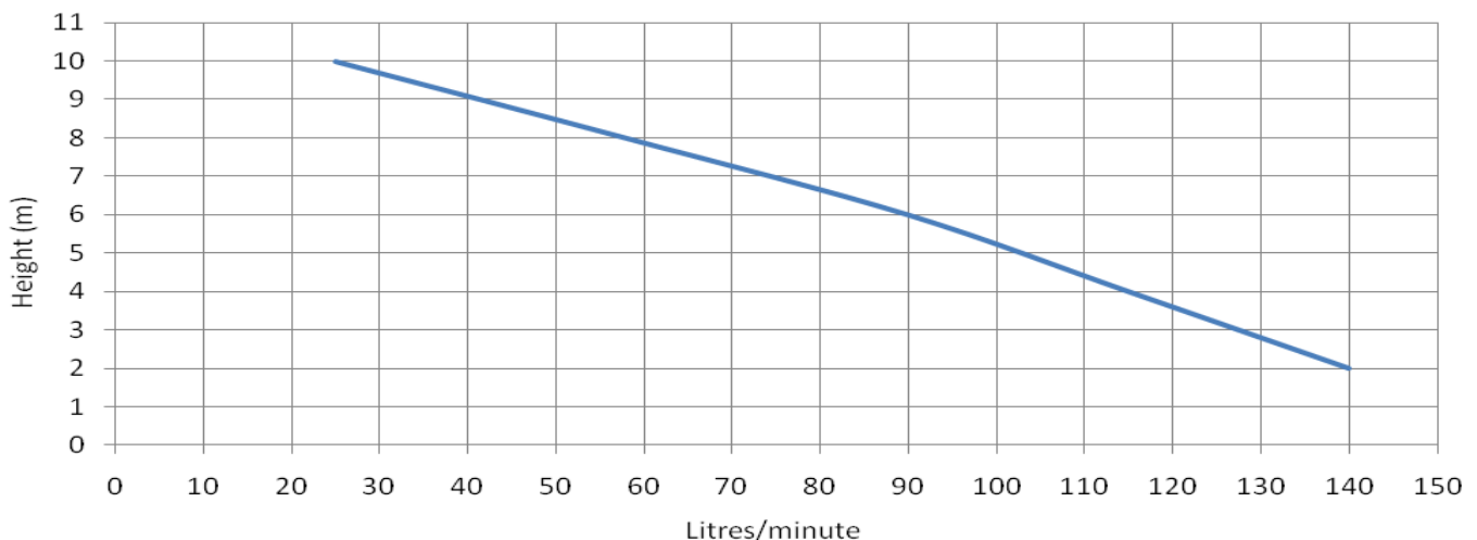
Pump Performance
