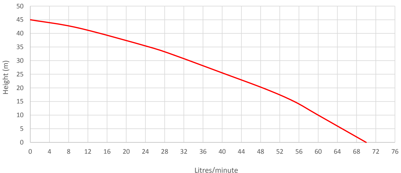
Pump Performance
