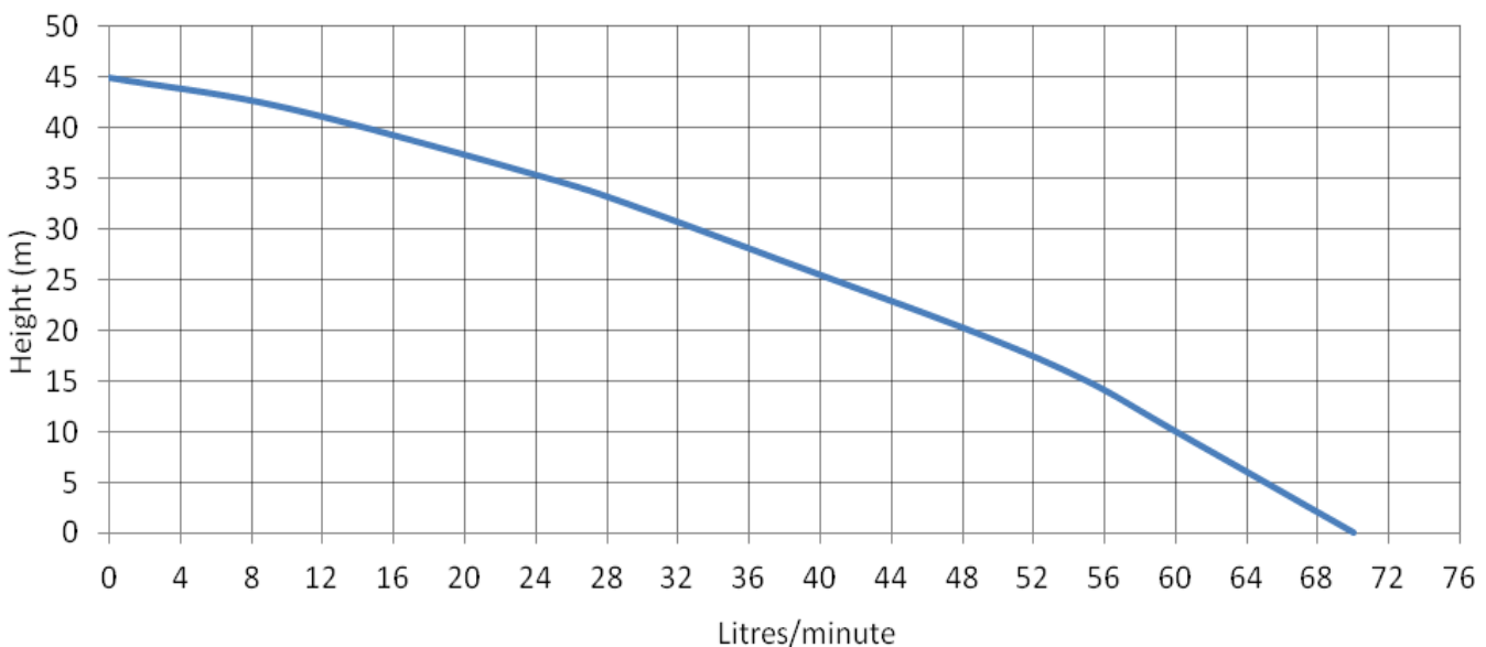
Pump Performance
