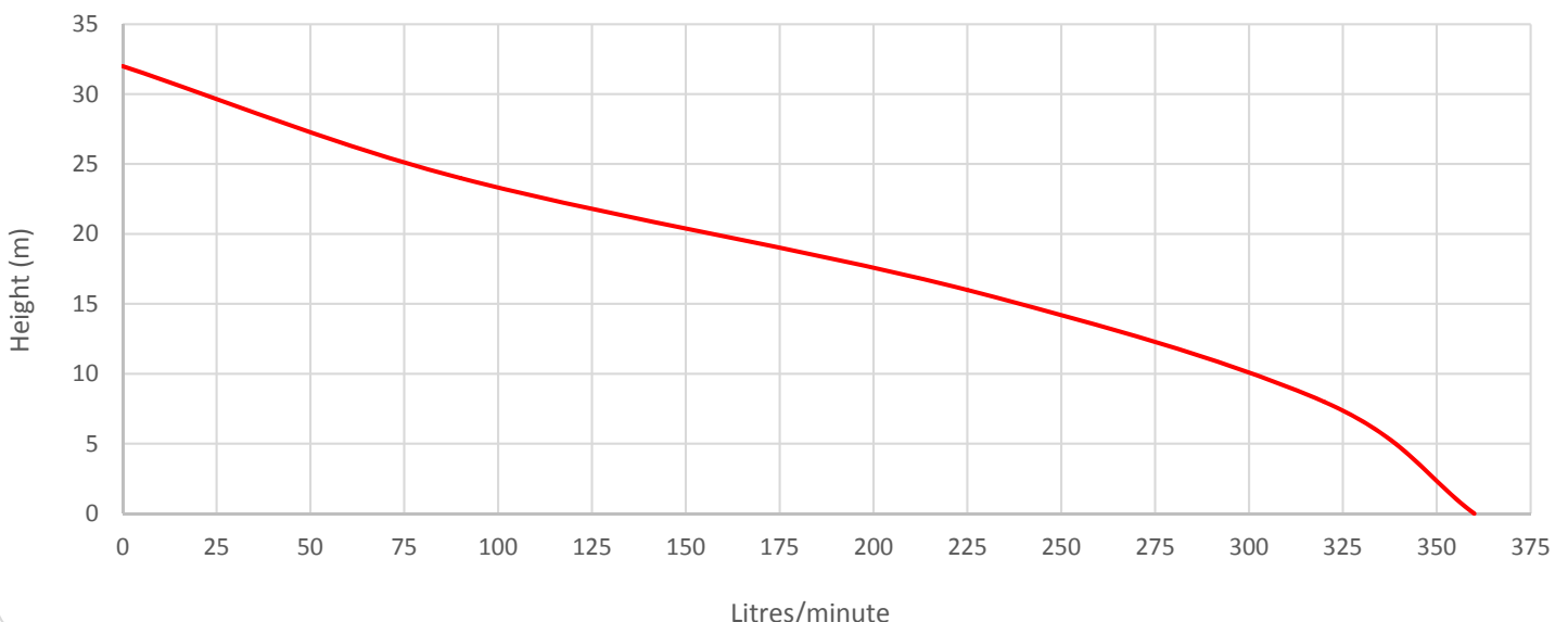
Pump Performance
