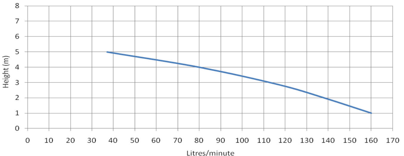
Pump Performance
